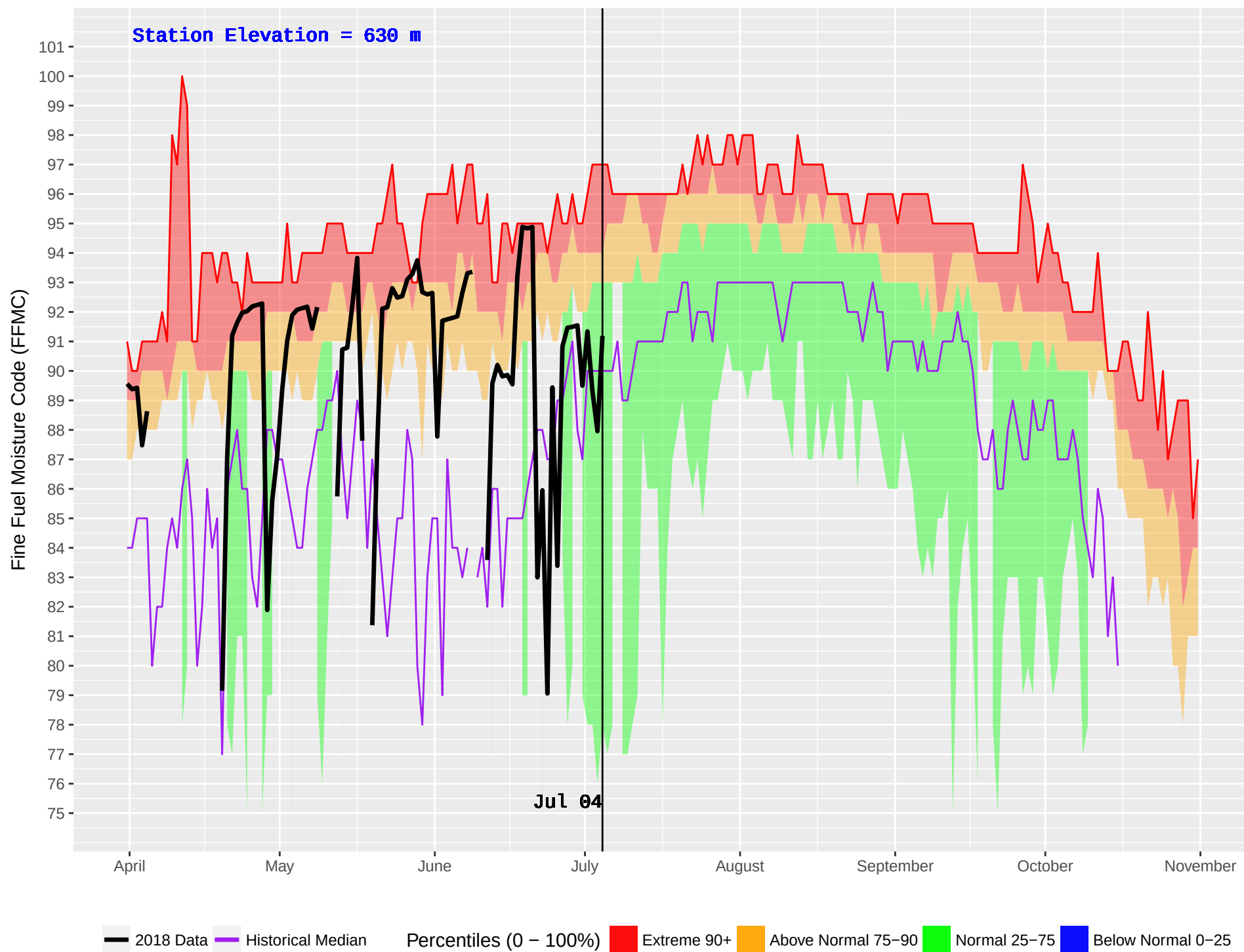
GRAND FORKS (392) : Historical (1981–2016) and Current (2018) Noon Fine Fuel Moisture Code (FFMC)
