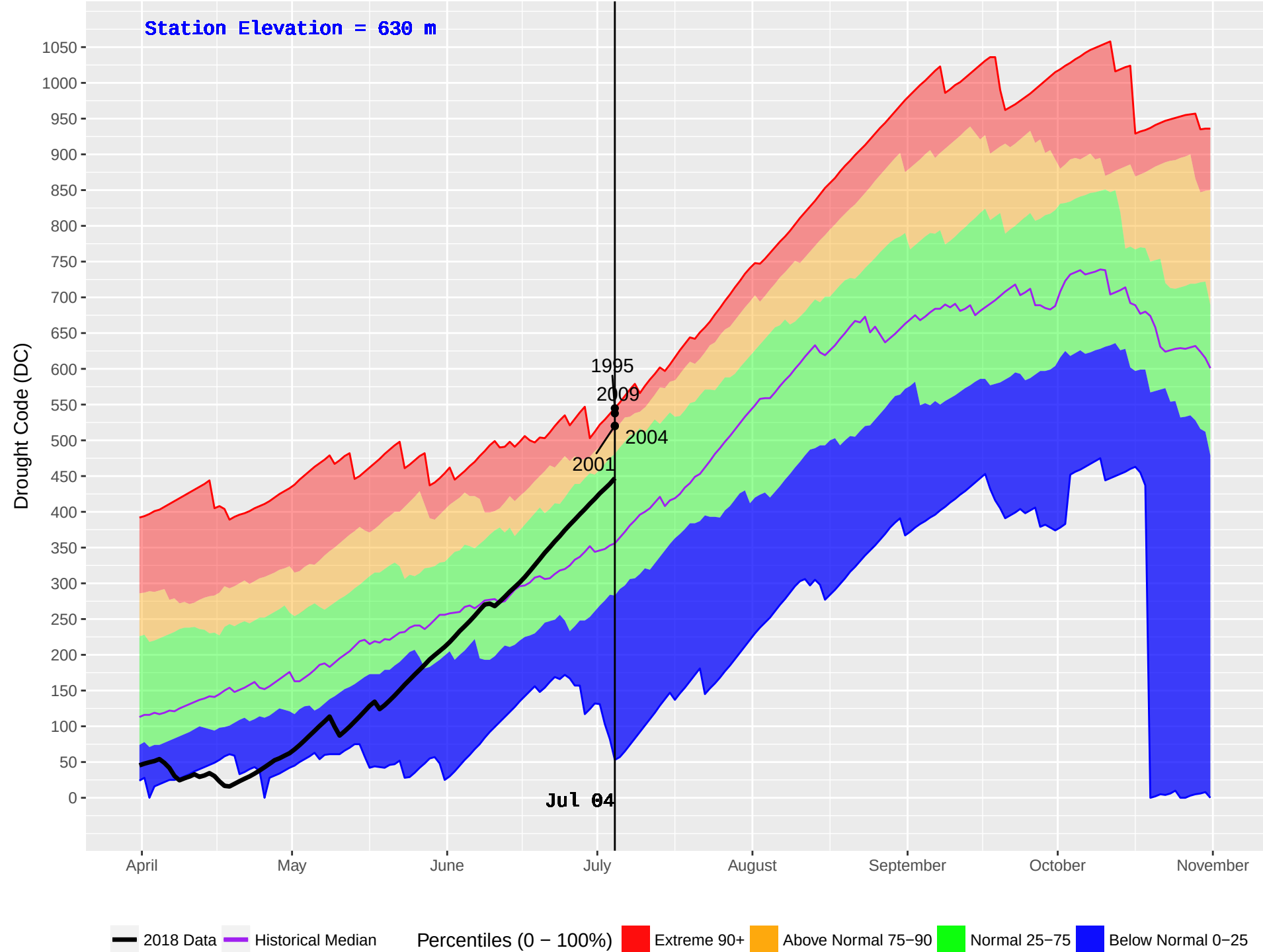
GRAND FORKS (392) : Historical (1981–2016) and Current (2018) Noon Drought Code (DC)
