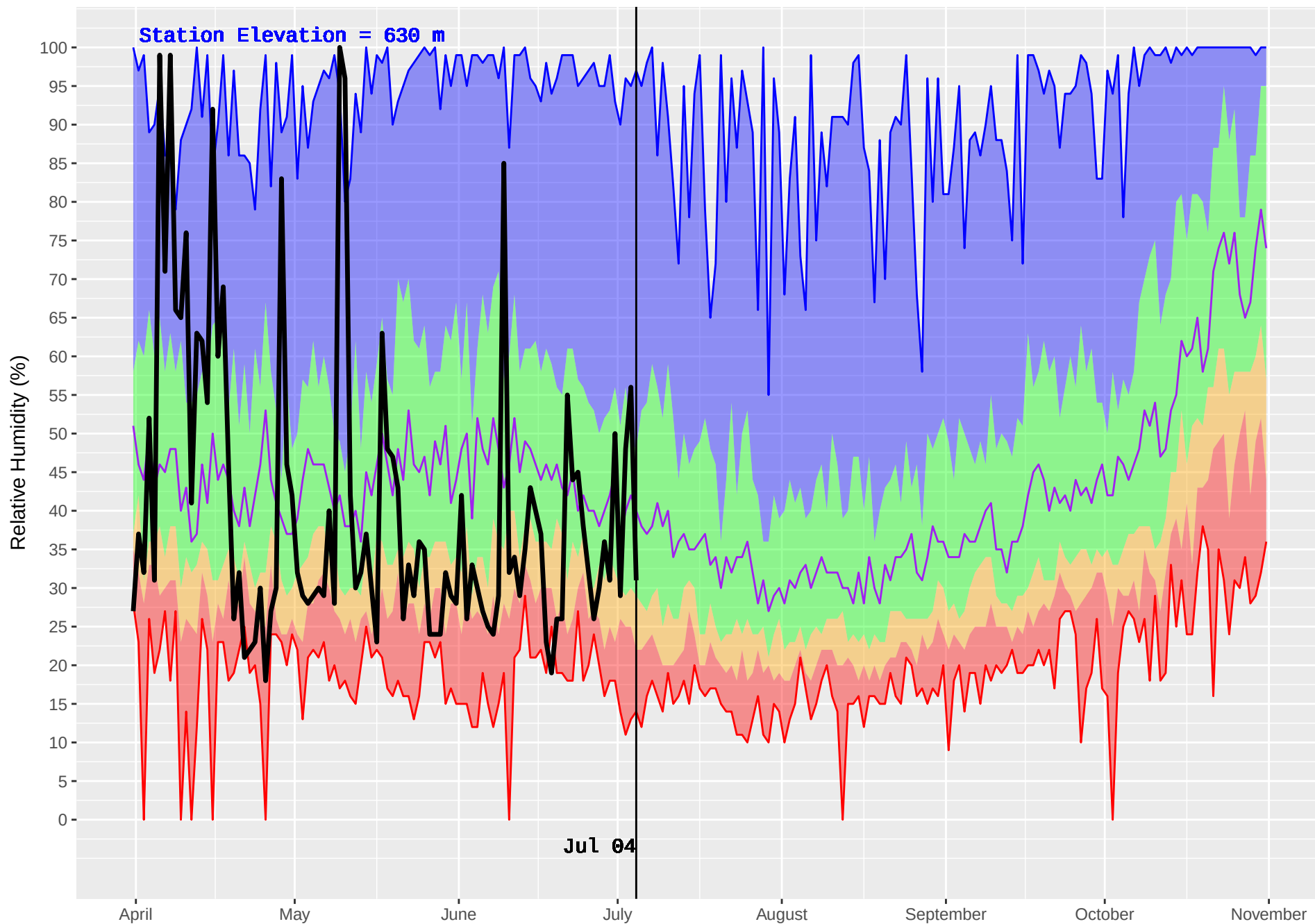
GRAND FORKS (392) : Historical (1981–2016) and Current (2018) Noon Relative Humidity
