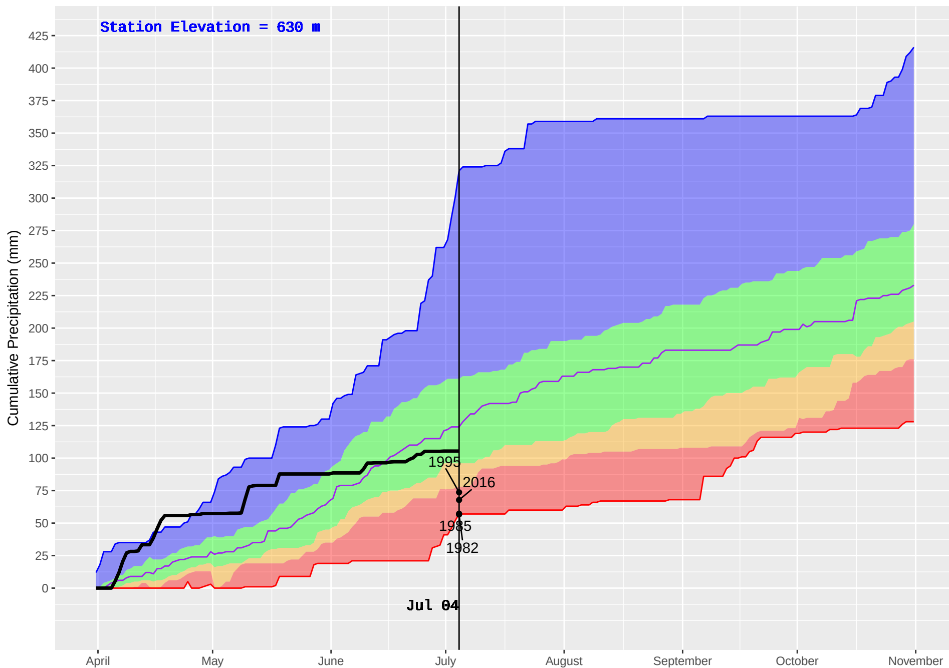
GRAND FORKS (392) : Historical (1981–2016) and Current (2018) Noon Cumulative Precipitation
