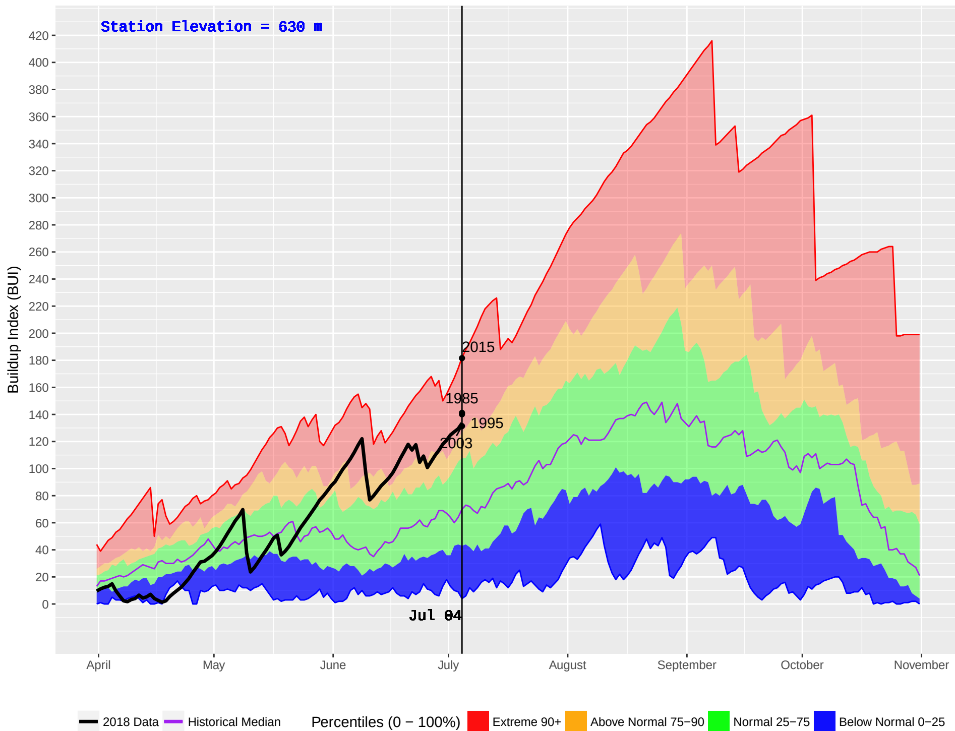
GRAND FORKS (392) : Historical (1981–2016) and Current (2018) Noon Buildup Index (BUI)
